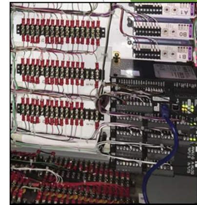
Space rocket lab test box build - reverse engineered from photos provided by customer
